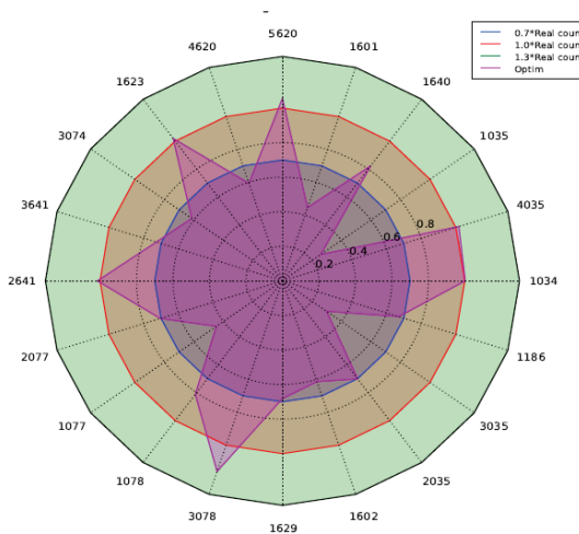
Figure 4: Calibration results star diagram. Each branch represents a sensor, whose simulated count should reach the red circle (normalized value of 1) corresponding to the average measured value. This solution, the best we obtained, corresponds to an average variance of 28%.
