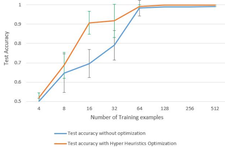
Fig. 7. Test accuracies with and without Hyper Heuristic Parameter Optimisation
