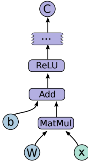
Fig. 5. A Tensorflow Computation Graph[2]
