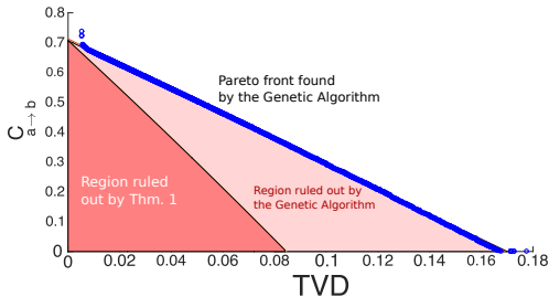
Figure 5. The Pareto front for the causal network in Figure 2c using the data from a photonic Bell experiment. The vertical axis labels the causal influence (9) while the horizontal axis labels the closeness to experimental data (7). The blue circles are the values for the non-dominated models found by the evolutionary algorithm. For comparison purposes, the straight line is a linear fit to these data.
