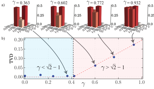
Figure 4. (a) The real component of experimentally measured density matrices for a range \gamma values measured via two-qubit state tomography. (b) the results of the MOEA (run as an EA) on a local model (see Figure 2a) to generate the best achievable TVD for various values of \gamma from a Bell-like experiment described in Section IV. As theoretically predicted above a certain threshold ( \gamma = \sqrt{2} - 1 ) the local model can no longer explain the measurement results with zero TVD. This threshold corresponds to violating the CHSH inequality in (15). The linear increase in TVD corresponds to the linear increase in S as discussed in Section IV.
