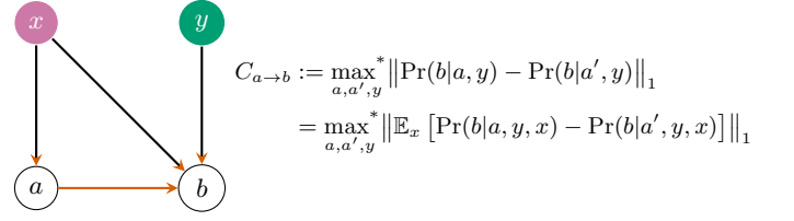
Figure 7. An example of the causal influence measure C_{a \rightarrow b}(I) given by (9) applied to a more complicated graph. The random variable y is conditioned on and maximized over, as it is a parent of b but not of a . By contrast, the variable x is also a parent of a and so it is marginalized over, resulting in the causal influence definition at right.
