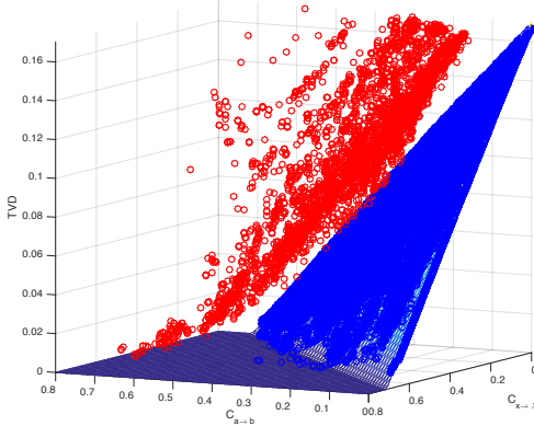
Figure 9. The 3D Pareto front for a \rightarrow b and x \rightarrow \lambda violations found using the “Island Model” is shown in blue. Beneath it is a linear mesh which fits the Pareto front with a Pearson’s \rho^2 of 0.9902. By Comparison the non-optimal Pareto front found by combining the best individuals from 8 runs using the basic algorithm (i.e. no pre-evolution) on the full graph is shown in red. The front shown in blue took a fraction of the computing time to find compared to the non-optimal red runs.
