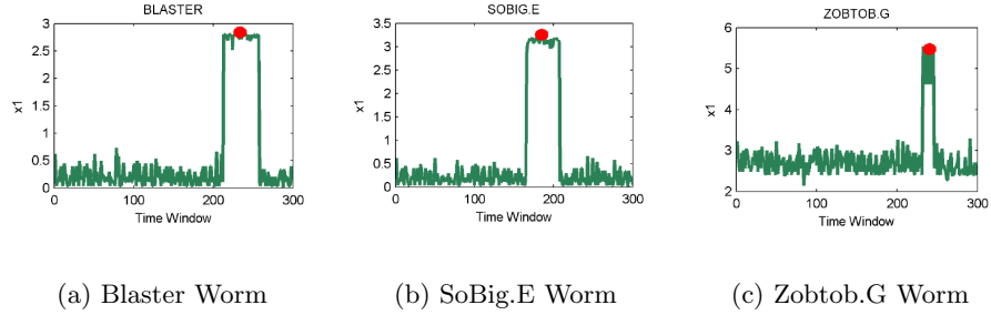
Fig. 2. Source Port Entropy for different worms
